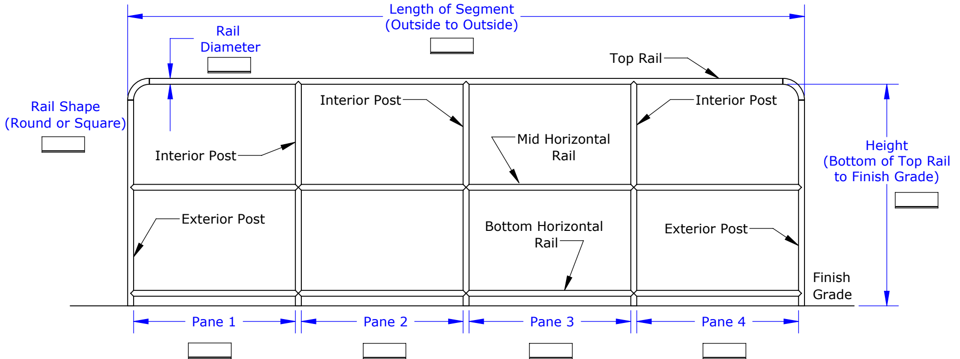
Guard Rail Segment as Viewed From Playing Field
