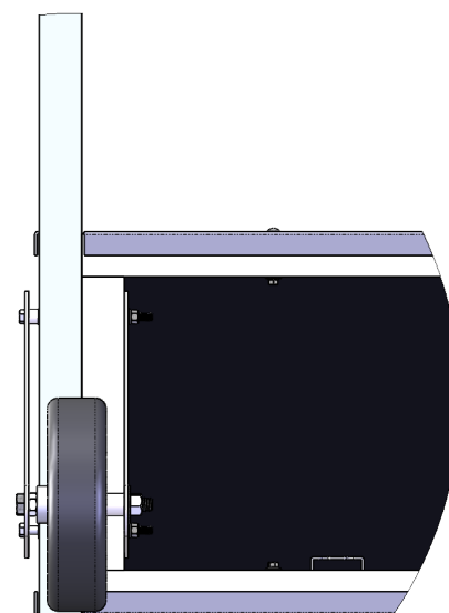
Back View Wheel Kit Assembly
