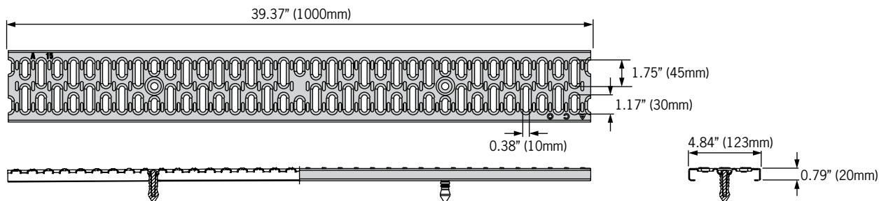
Side elevation
