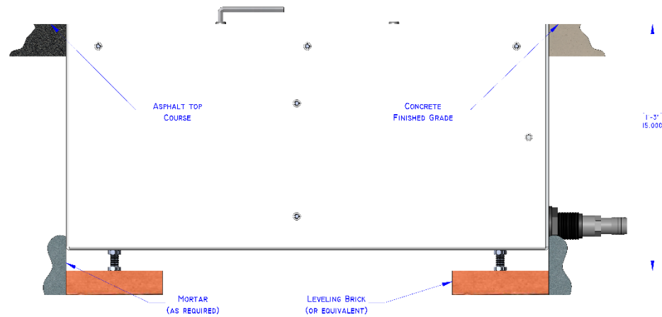
Diagram 1 Combox® elevation detail.
